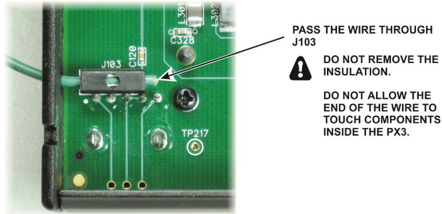
Figure 19. Calibrator Signal Pickup Wire Installed in the PX3.
