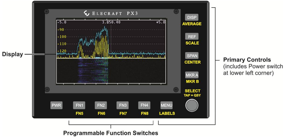
Figure 4. PX3 Control Groups.
