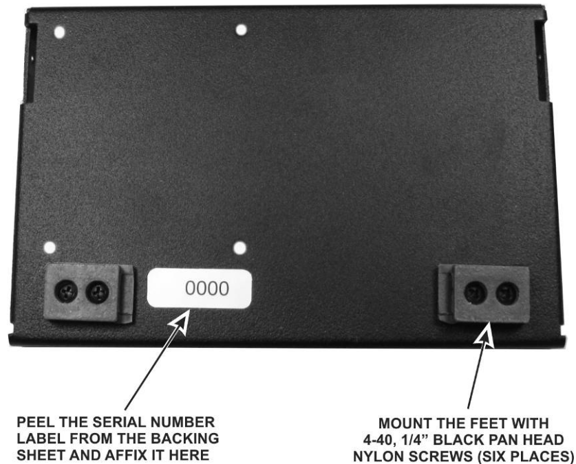
Figure 41. Installing Fixed Feet and Serial Number on Bottom Cover.
