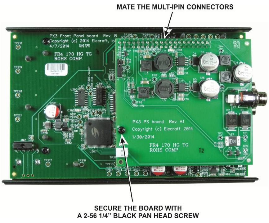
Figure 32. Installing the Power Supply Board.
