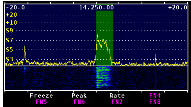
Figure 10. Bar Cursor on Upper Sideband Signal at 14.250 kHz.
