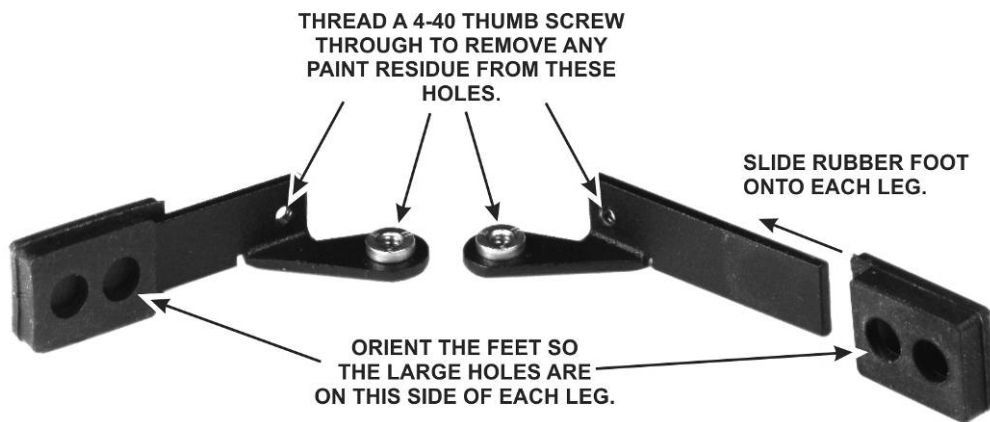
Figure 38. Preparing the Tilt Legs for Installation.
