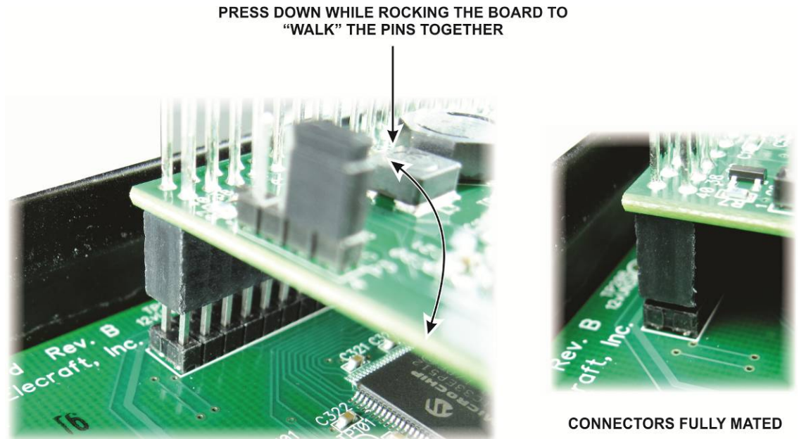
Figure 33. Mating the Power Supply Board Connectors.
