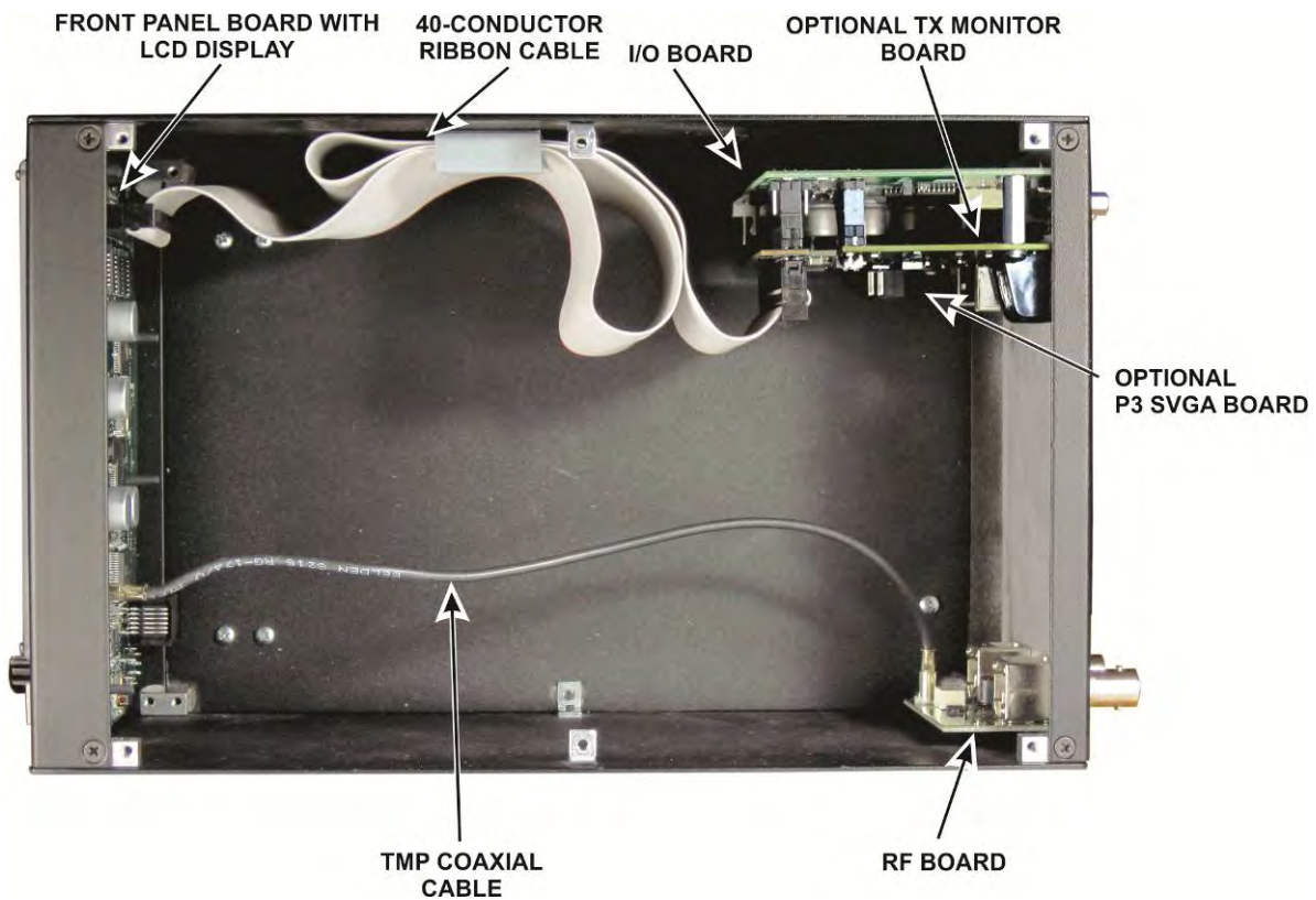
Figure 1 Assembled P3 with Top Cover Removed.
