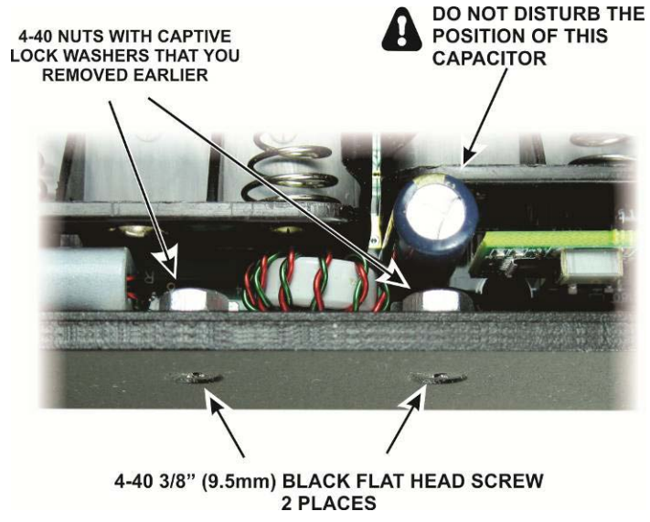
Figure 46. Securing the Tabs for Q6 and Q7 on the RF Board to the Bottom Cover.
