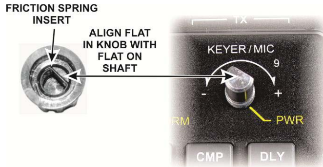
Figure 21. Mounting Friction Knobs.
