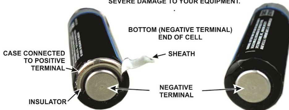
Figure 60. Checking Battery Cells.
