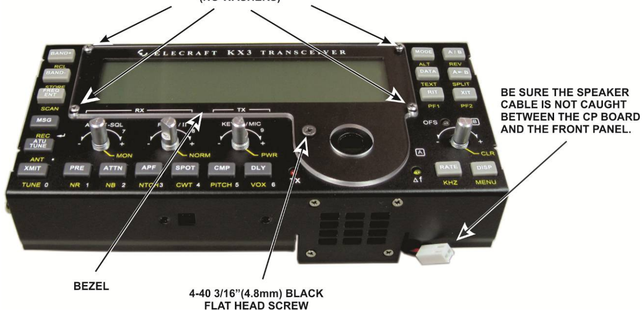
Figure 14. Placing the CP Board in the Front Panel.
