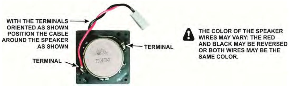
Figure 7. Dressing the Speaker Cable.
