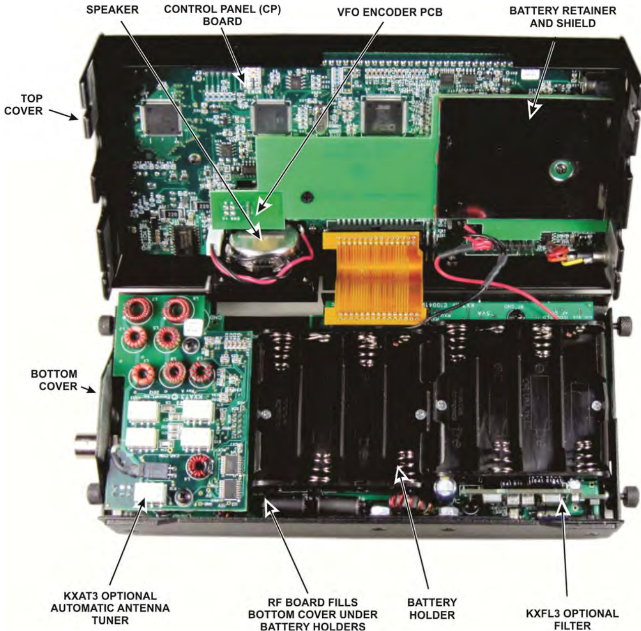
Figure 1. Complete KX3.
