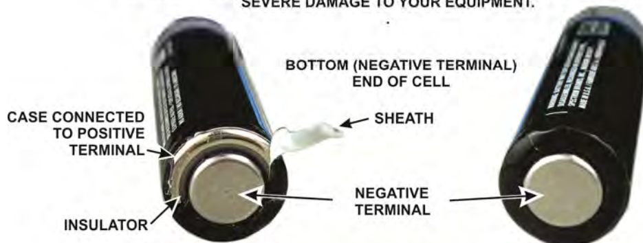
Figure 55. Checking Battery Cells.
