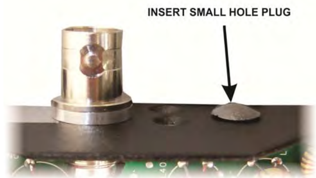
Figure 42. Installing the Hole Plug.
