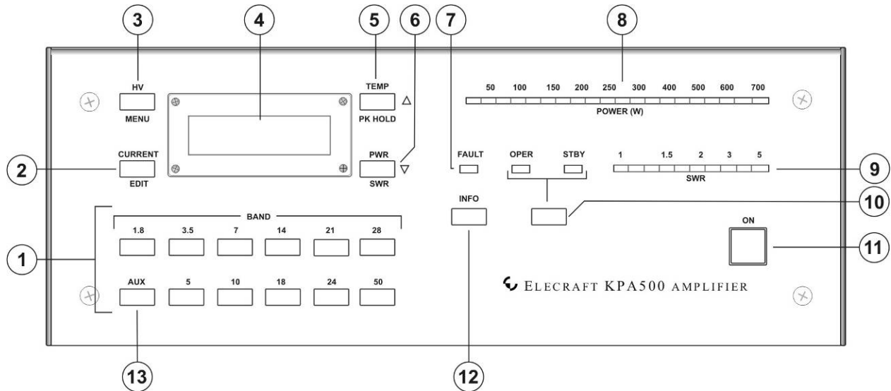
Figure 5. KPA500 Front Panel.
