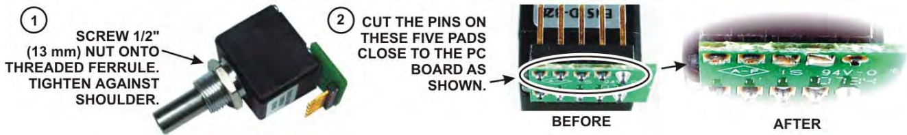
Figure 43. VFO B Encoder Assembly Preparation for Installation.
